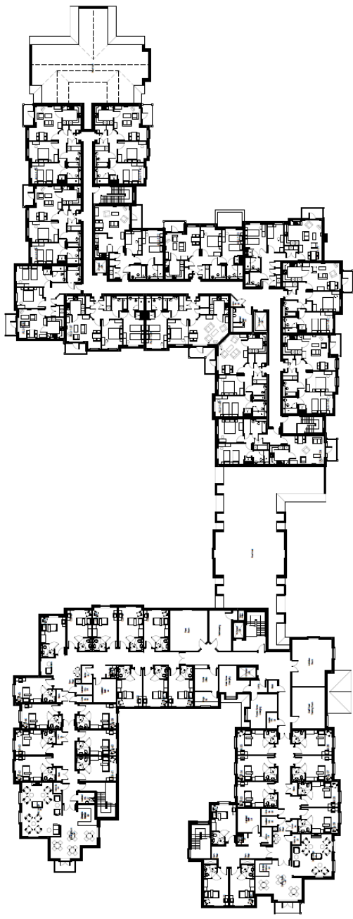
First Floor Plan CARE HOME VILLAGE CARE CENTRE
